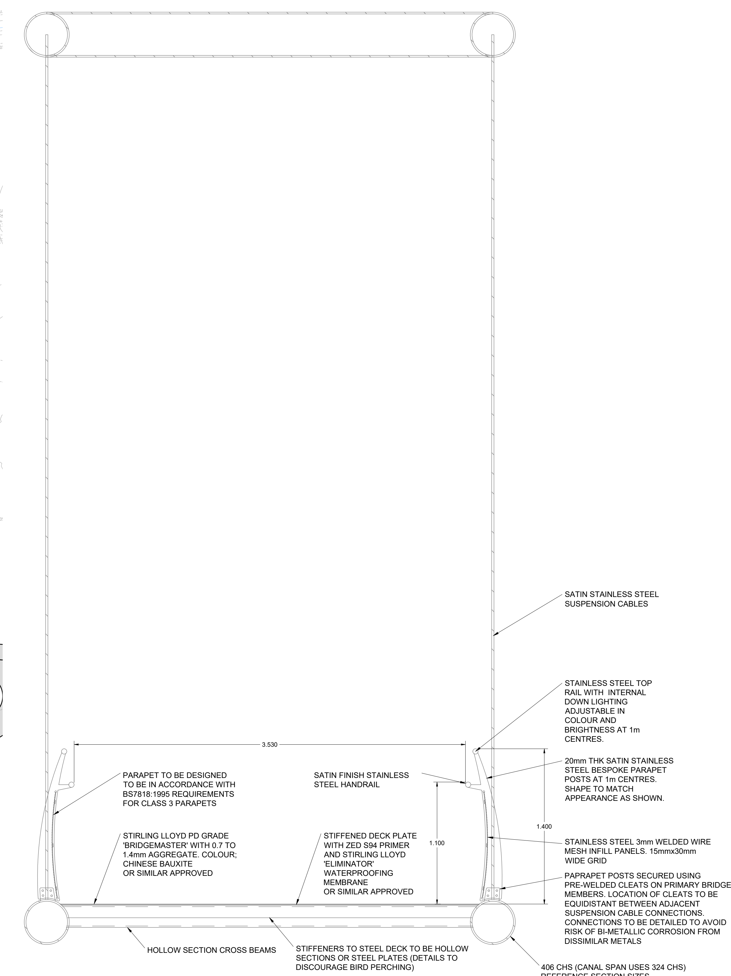
TIED ARCH BRIDGE DECK TYPICAL SECTION - MAIN RIVER SPAN - CHAINAGE 88.97m Scale 1:20
