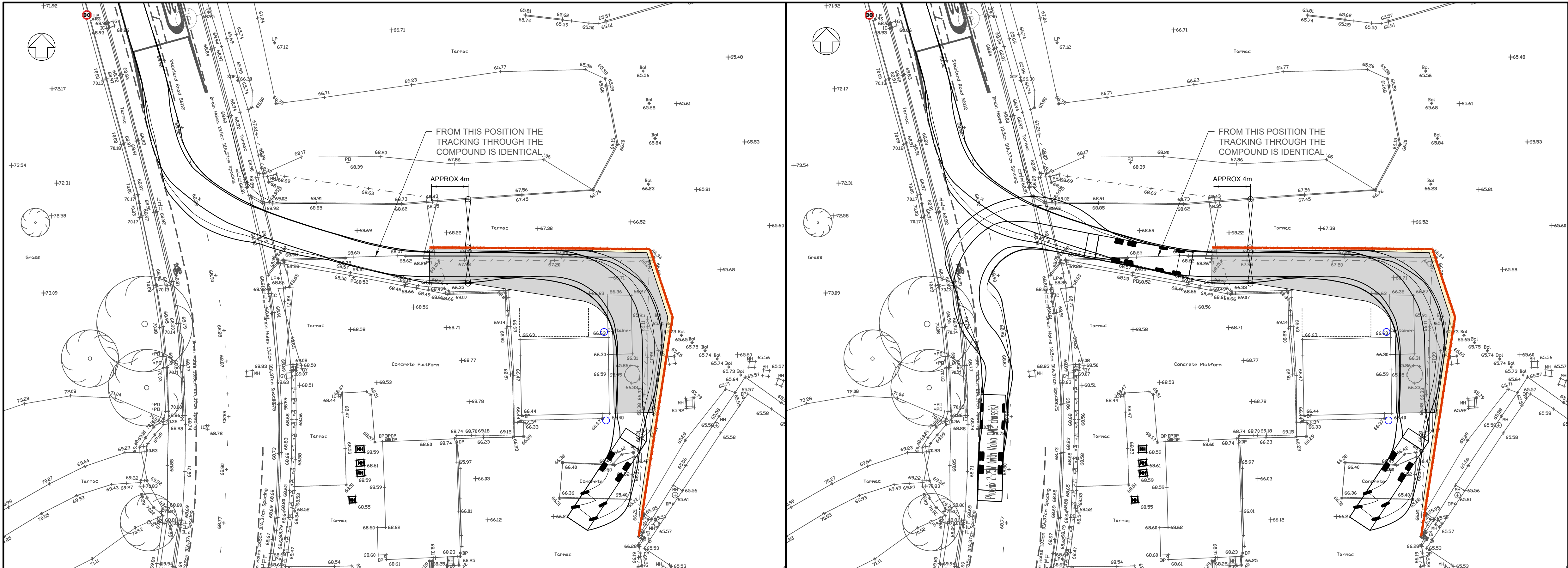
ACCESS FROM SOUTHBOUND CARRIAGEWAY SCALE 1:250
