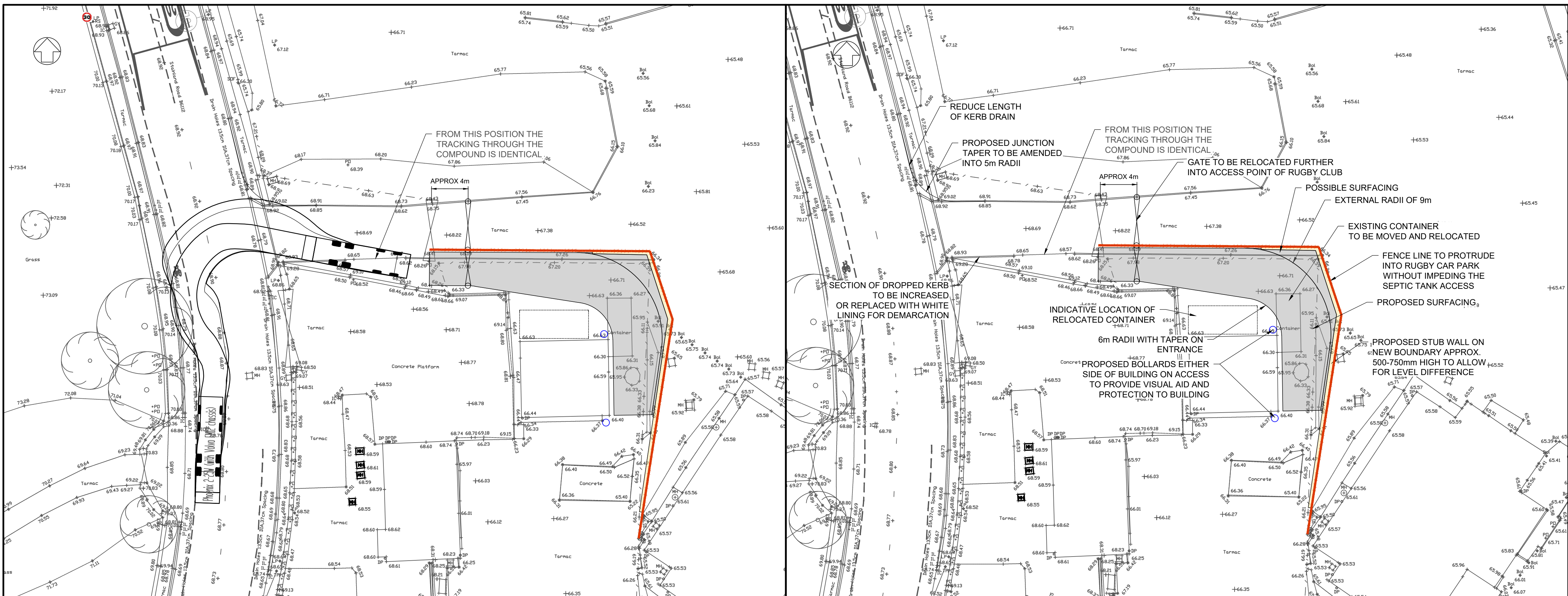
ACCESS FROM NORTHBOUND CARRIAGEWAY SCALE 1:250
